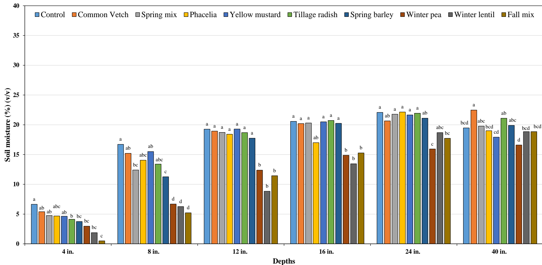
Figure 2: Residual soil moisture levels at different depths after cover crop termination in Morrow County, Oregon, USA. Different letters denote statistically different means within each depth based on Least Square Difference (LSD) at p \leq 0.05 .
