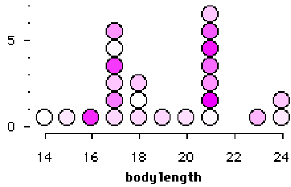
Figure 5. Body length of cats with data icons shaded according to age such that the older the cat, the darker its icon.
