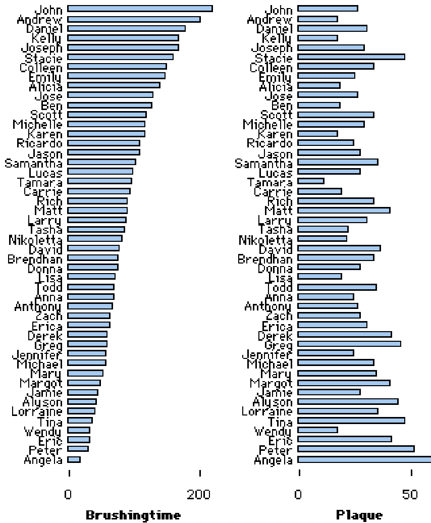
Figure 3. Paired case-value plots showing time in seconds spent brushing (left) and percent of remaining plaque (right). Knowing that the bars are ordered according to brushing time, you can determine the effects of increasing brushing time by tracking the changing lengths of the “plaque” bars as you visually scan them from bottom to top.
