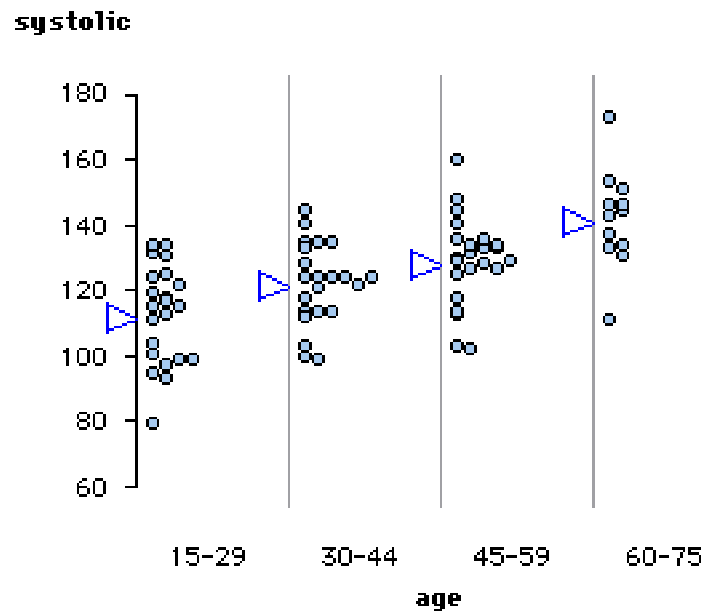
Figure 2. Systolic blood pressure of people grouped in various age categories. Adapted from Noss, Pozzi, and Hoyles (1999). The triangles show the location of the mean blood pressure in each age grouping.
