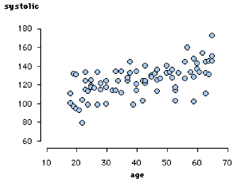
Figure 1. Scatterplot of age and systolic blood pressure, adapted from data reproduced in Noss, Pozzi, and Hoyles (1999).
