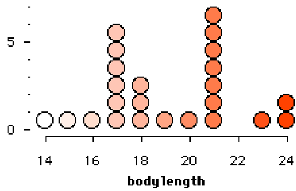
Figure 4. Body length of 24 cats with data icons shaded according to body length such that the longer the cat, the darker its icon.
